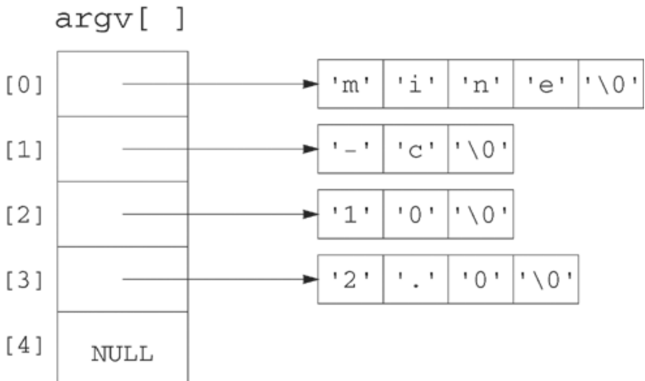
Figure 2.2. The argv array for the call mine -c 10 2.0 .
